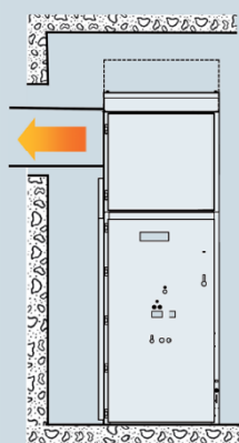
Lateral pressure relief duct
